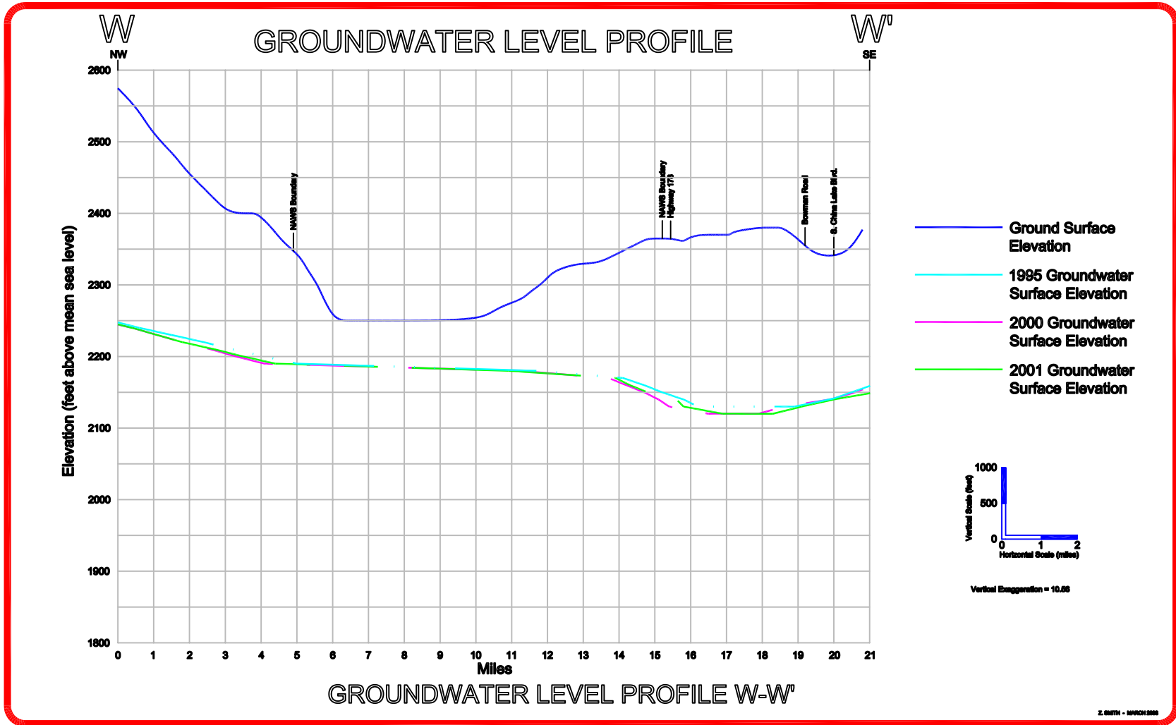
INDIAN WELLS VALLEY BASIN, CALIFORNIA FIGURE 3-14 GROUNDWATER LEVEL PROFILE W-W' FOR THE REGIONAL AQUIFER, 2000 AND 2001 KERN COUNTY WATER AGENCY
