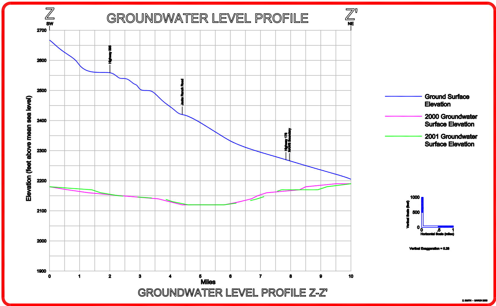
INDIAN WELLS VALLEY BASIN, CALIFORNIA FIGURE 3-17 GROUNDWATER LEVEL PROFILE Z-Z' FOR THE REGIONAL AQUIFER, 2000 AND 2001 KERN COUNTY WATER AGENCY
